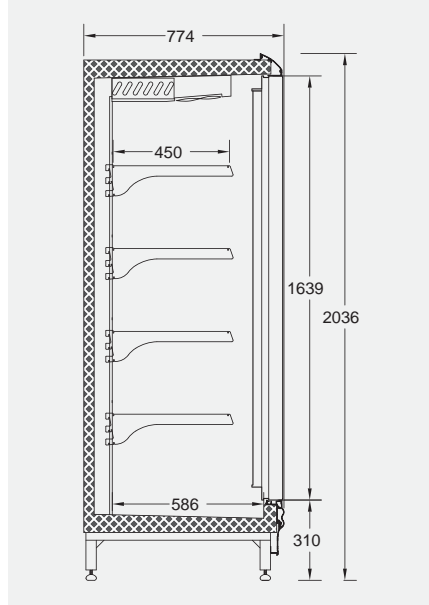
Çiğdem Kapaklı / Crocus Hinged Door
